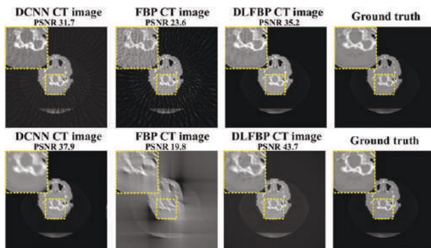
Fig. 18.7 Deep learning-based sinogram completion for sparse ( top ) and limited-angle ( bottom ) CT scans. DCNN deep convolutional neural network (Jin et al. 2017), FBP filtered backprojection, DLFBP deep learning filtered backprojection (Dong et al. 2019), PSNR peak signal-to-noise ratio. (Reproduced from Dong et al. 2019 under a Creative Commons Attribution License)
