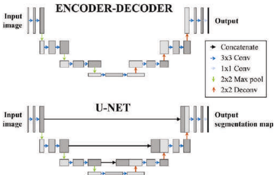
Fig. 17.1 Examples of a typical encoder-decoder (top) and U-Net (bottom) architecture
