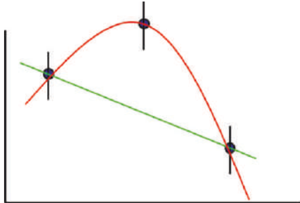
Half-Factorial, 3-Factor Experiment ( 2^{3-1} designs)
