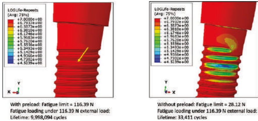
Fig. 6.7 Effect of connector screw preload on fatigue lifetime as predicted by the FEA post-processor (fe-safe). The heat shows the expected failure time for each location on the implant with cool colors (blue) indicating short lifetime and hot colors (red) indicating long lifetime. With permission from (Satpathy et al. 2022a,b)
