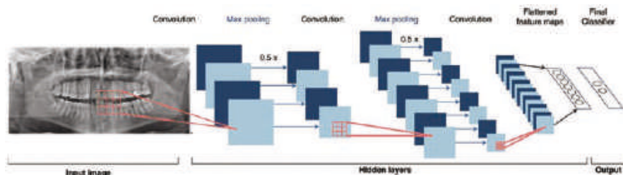
Fig. 2.5 How building blocks outlined in this chapter is organized into deep neural architectures
